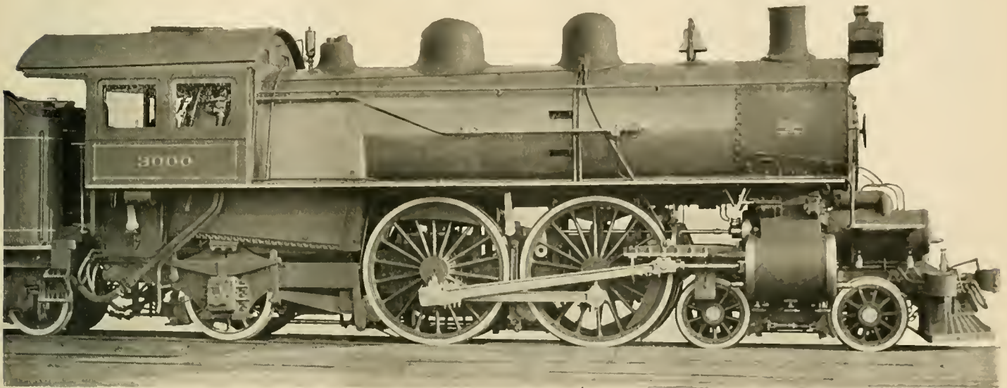
FOUR-CYLINDER, BALANCED, DIVIDED COMPOUND LOCOMOTIVE—44-2 TYPE.—NEW YORK CENTRAL & HUDSON RIVER RAILROAD. J. F. Deems, General Superintendent Motive Power. American Locomotive Company, Schenectady Works, Builders.
